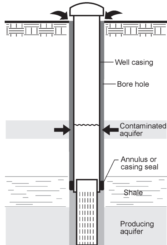
Figure 1 Annular or Casing Seal
