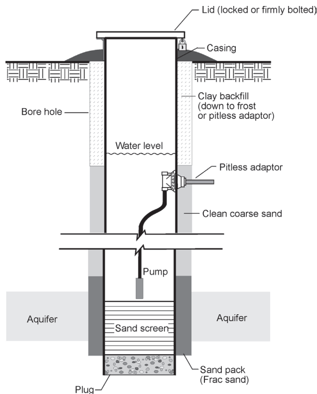
Figure 1 Bored Well
